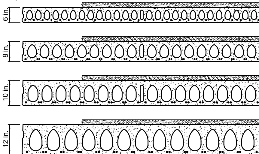
Standard Spancrete®
