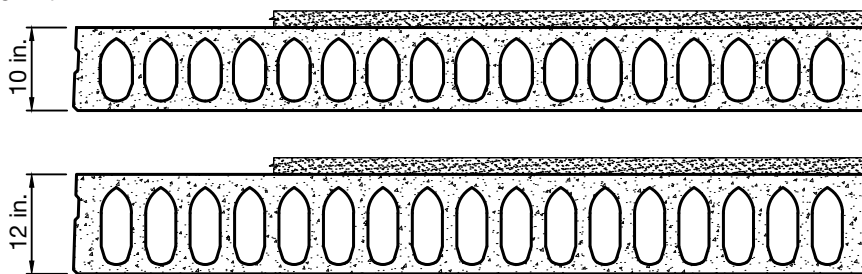
Ultralight Spancrete®
